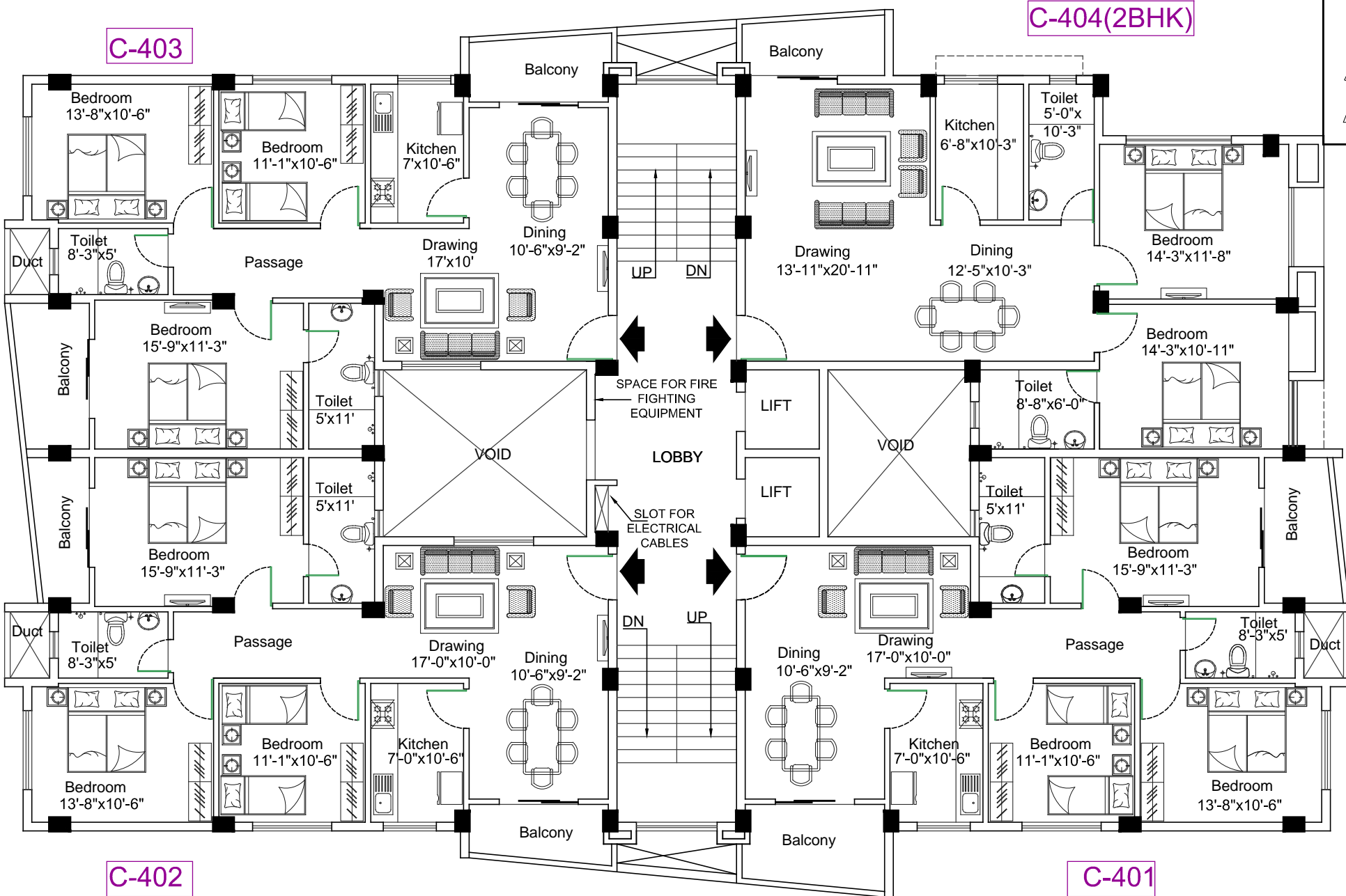
BLOCK - C 4TH FLOOR PLAN.
