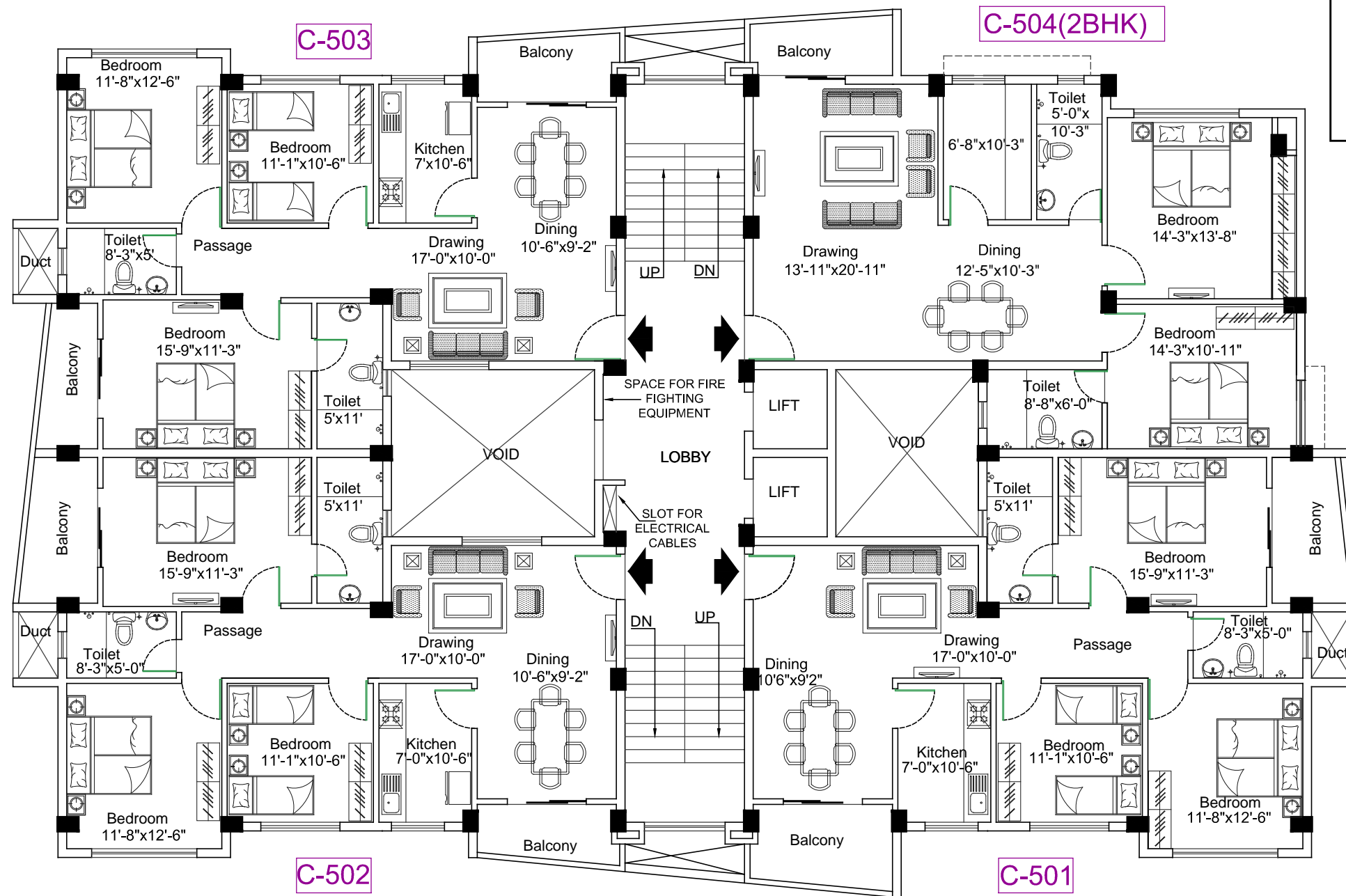
BLOCK - C 5th FLOOR PLAN.
