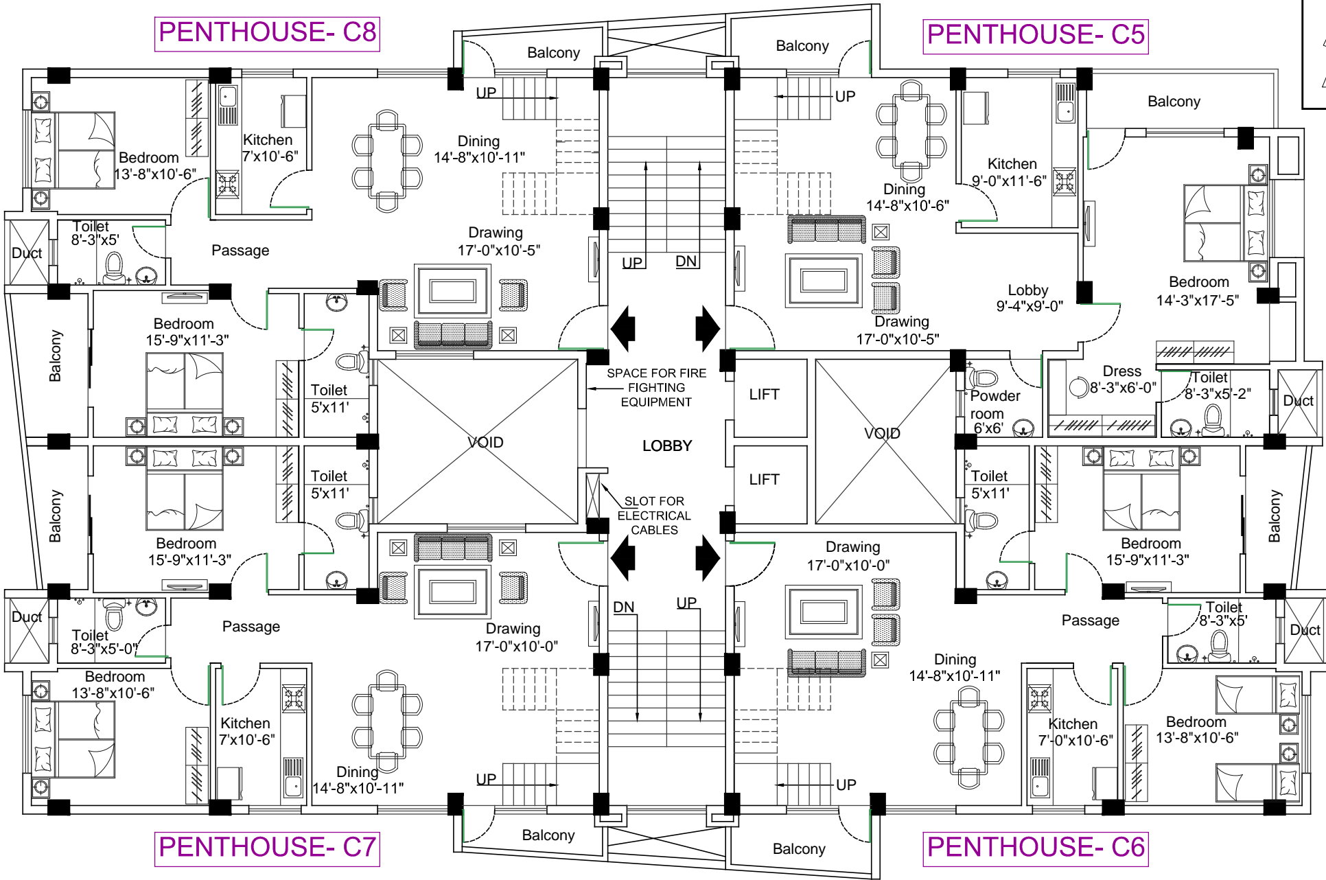
BLOCK - C 8th FLOOR PLAN
