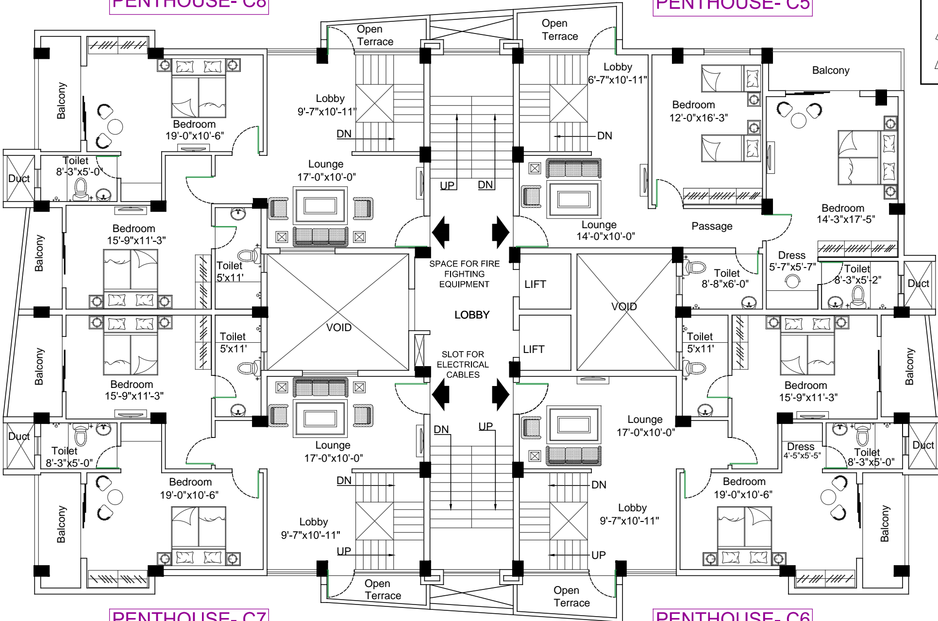
BLOCK - C 9th FLOOR PLAN
