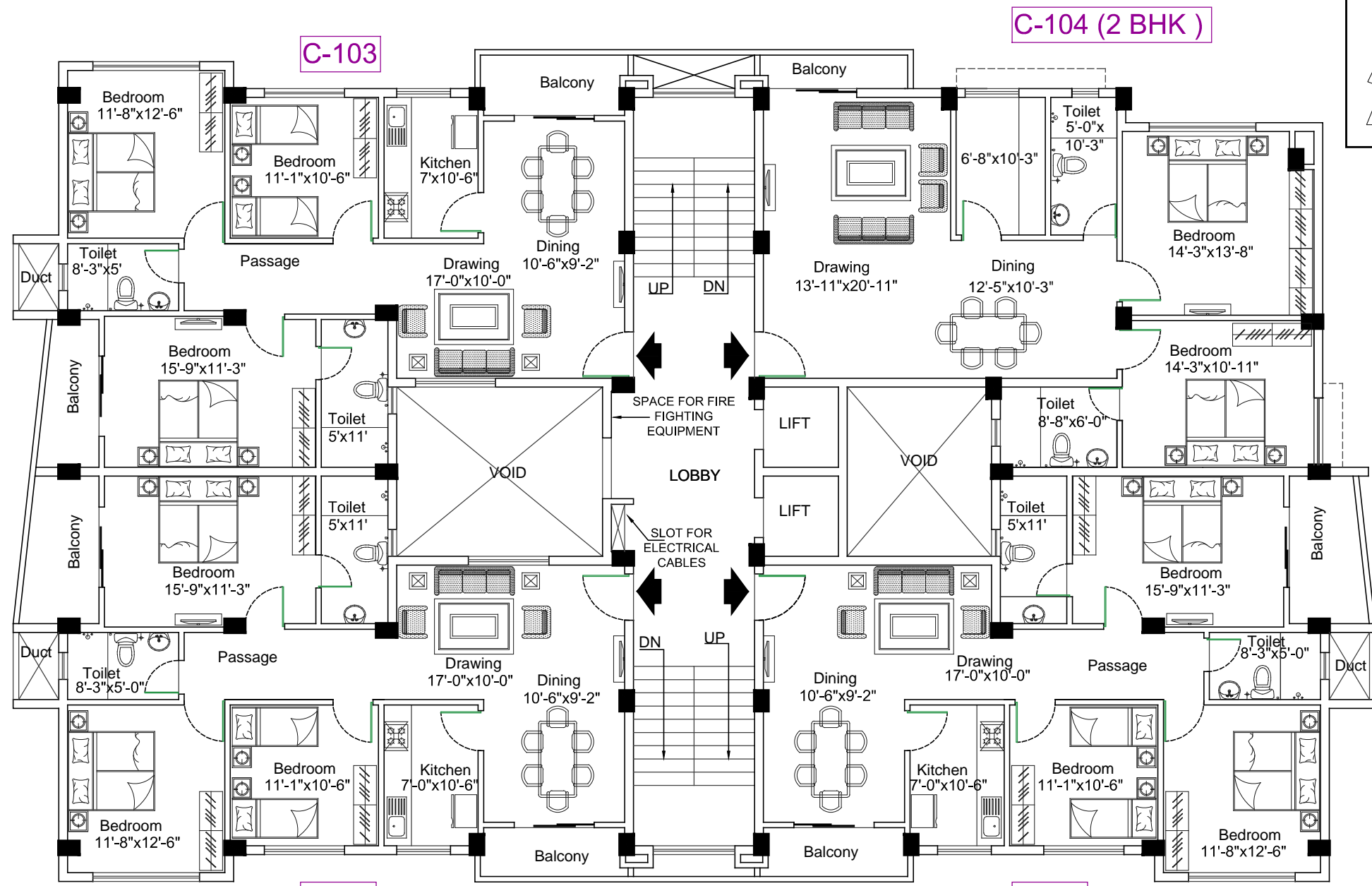
BLOCK - C FIRST FLOOR PLAN
