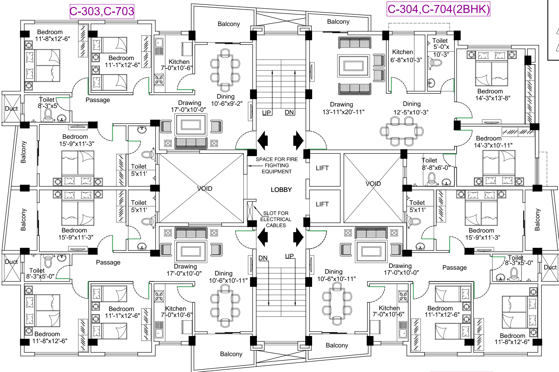
BLOCK - C TYPICAL FLOOR 3rd & 7th.
